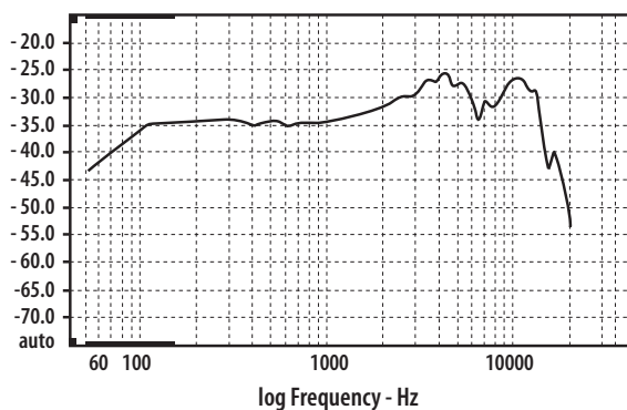
Transfer Function Mag - dB volts/volts (0.10 oct)
